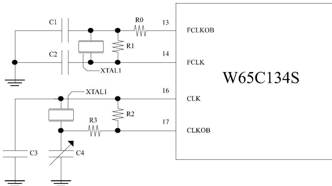
Figure 8.2-1 Oscillator Circuit
